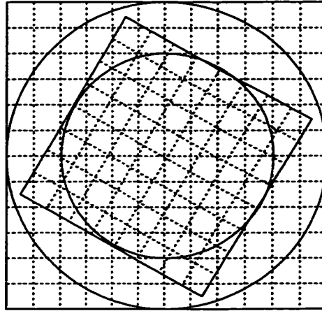
Figure 2.7: The small 8 \times 8 pixel square shows the size of the sky viewed by the imager at one instant. The large circle shows the area of sky viewed by the imager in one revolution. The small circle shows the area of sky that is continuously viewed by the imager.
