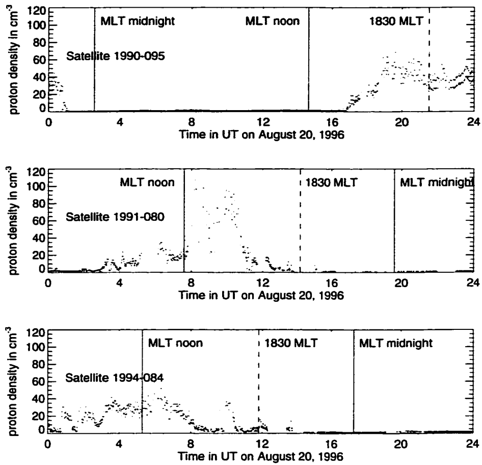
Figure 3.18: Low energy (1-130 eV) proton densities from the MPA instrument on the LANL geosynchronous satellites, from the NASA CDA web site, courtesy of D. McComas.
