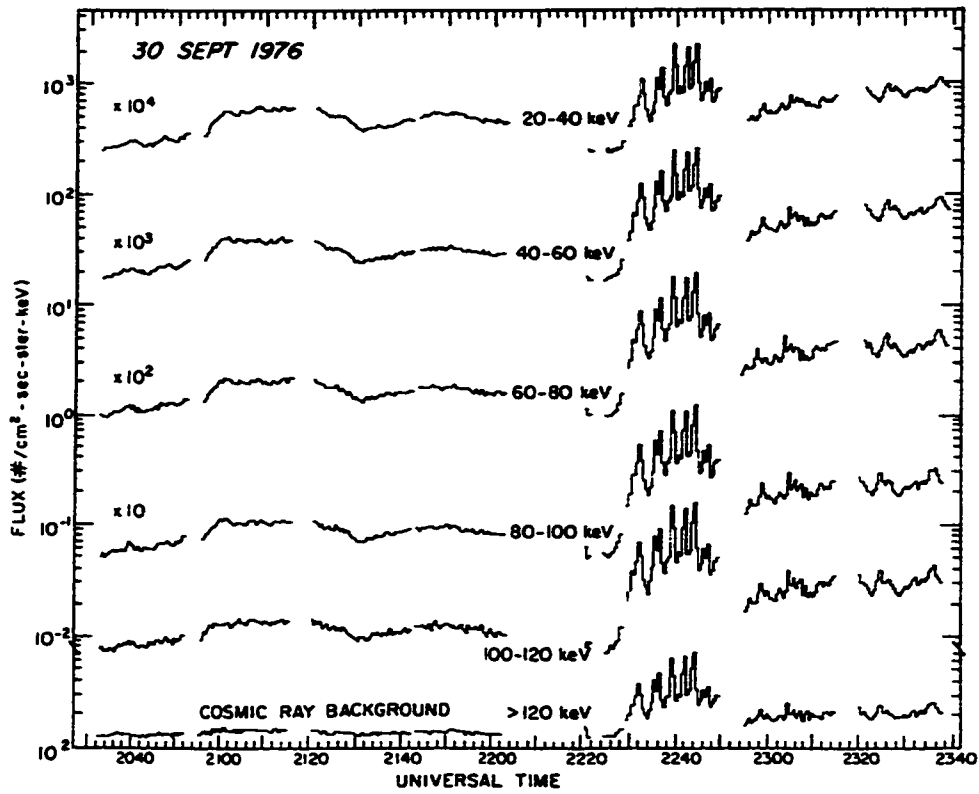
Figure 1.4: Previous balloon X-ray observations of a dayside REP event from West and Parks [1984].
