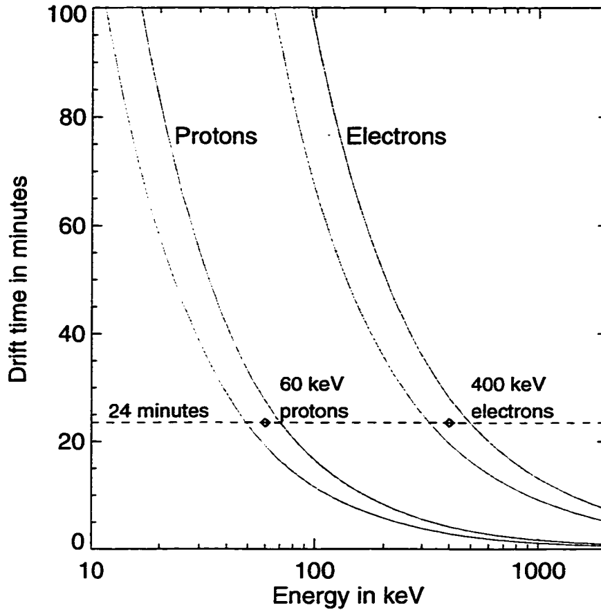
Figure 4.11: Gradient-curvature drift times in minutes for particles drifting around the Earth at L = 6 , from the LANL satellite 1991-084 at 175^\circ magnetic longitude (near midnight) to the balloon field line at 118^\circ magnetic longitude (near dusk). The shaded region of each curve gives the range of drift times for \alpha \approx 0^\circ to \alpha \approx 90^\circ .
