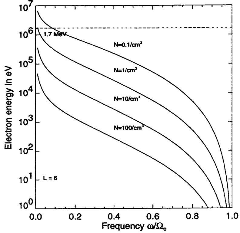
Figure 4.3: Electron parallel resonance energy for various densities and whistler wave frequencies calculated using the low-gamma approximation from Equation 4.7.
