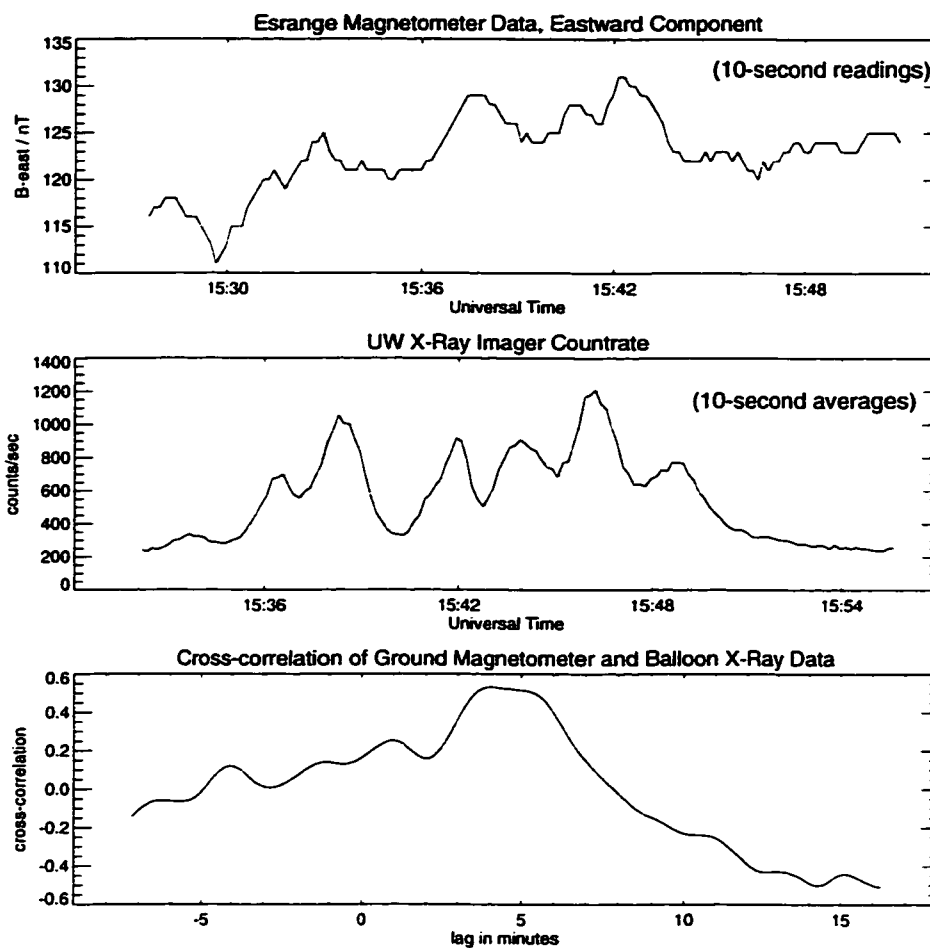
Figure 4.10: Cross-correlation between field line resonances and X-ray bursts reveals that the data agree best with a 4-minute time lag.
