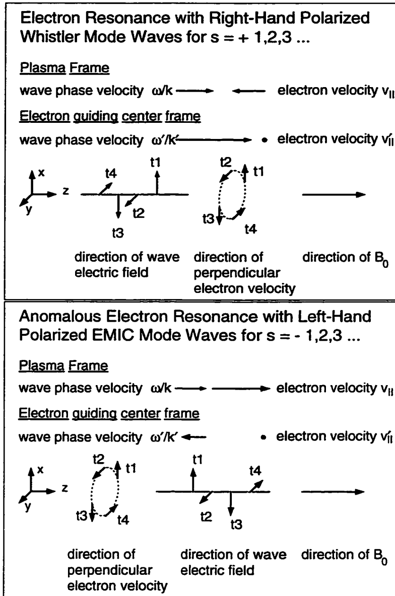
Figure 4.1: Electron resonance for regular and anomalous Doppler shifts. The top panel shows how an electron can resonate with a right-hand polarized whistler mode wave. The bottom panel shows how an electron can resonate with a left-hand polarized EMIC mode wave.
