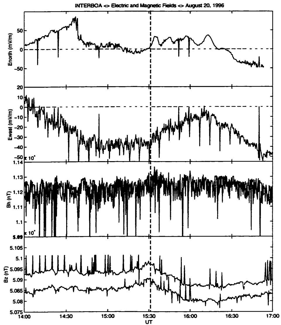
Figure 3.7: Electric and magnetic field data from balloon instruments, courtesy of J. P. Treilhou, CESR, Toulouse, France. The large spikes are due to data problems and are not real. Northward electric field data show oscillations with periods of 7-8 minutes starting at 1530 UT. The start of the REP event at 1532 UT is indicated with a dashed vertical line.
