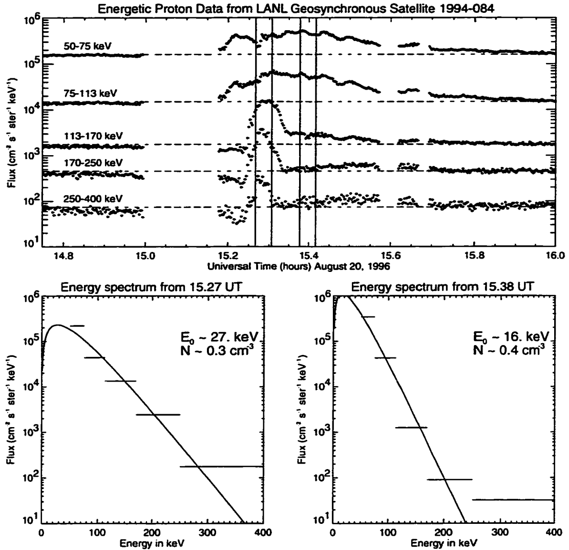
Figure 5.2: Proton injection data from LANL geosynchronous satellite 1994-084. The top panel shows the proton flux during the substorm injection. The horizontal dashed lines give the background flux, determined from 1423 to 1458 UT. The solid vertical lines identify the 2.5 minute intervals shown in the bottom two panels. These two panels show background-subtracted spectra and a least squares fit to E \exp(-E/E_0) for the four lowest-energy channels.
