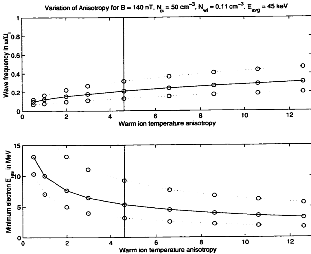
Figure 5.10: Wave frequency and electron resonance energy vs. warm ion anisotropy. The vertical line shows the parameters used to determine the wave growth shown previously in the bottom of Figure 5.5.
