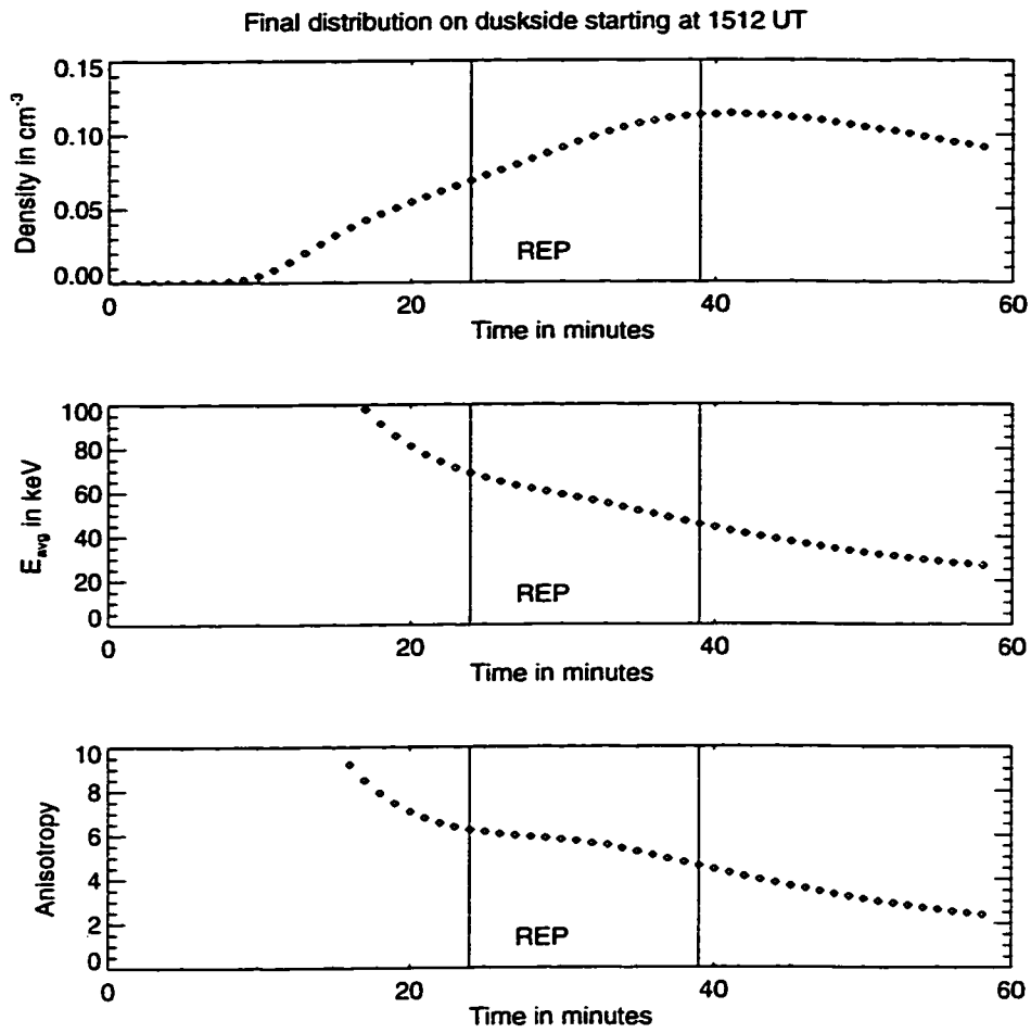
Figure 5.4: Final duskside results for the density, average energy and temperature anisotropy of the proton drift simulation.
