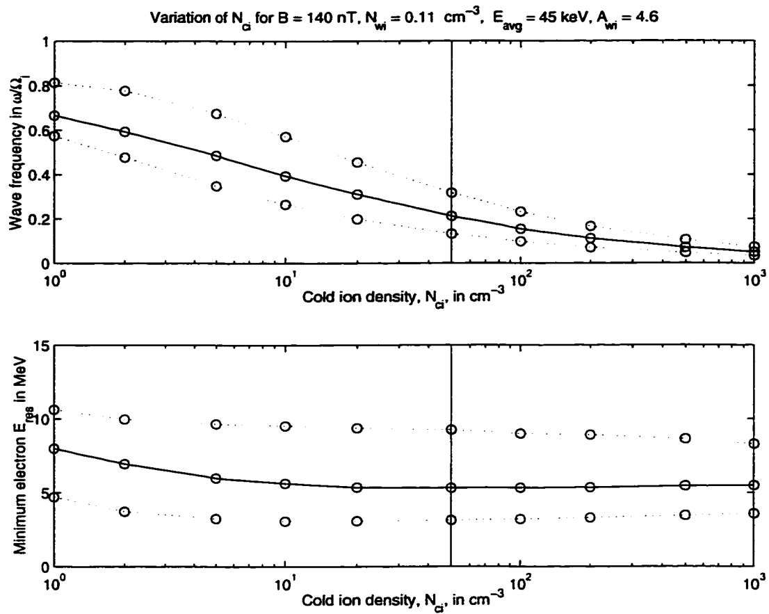
Figure 5.7: Wave frequency and electron resonance energy vs. cold ion density. The vertical line shows the parameters used to determine the wave growth shown previously in the bottom of Figure 5.5.
