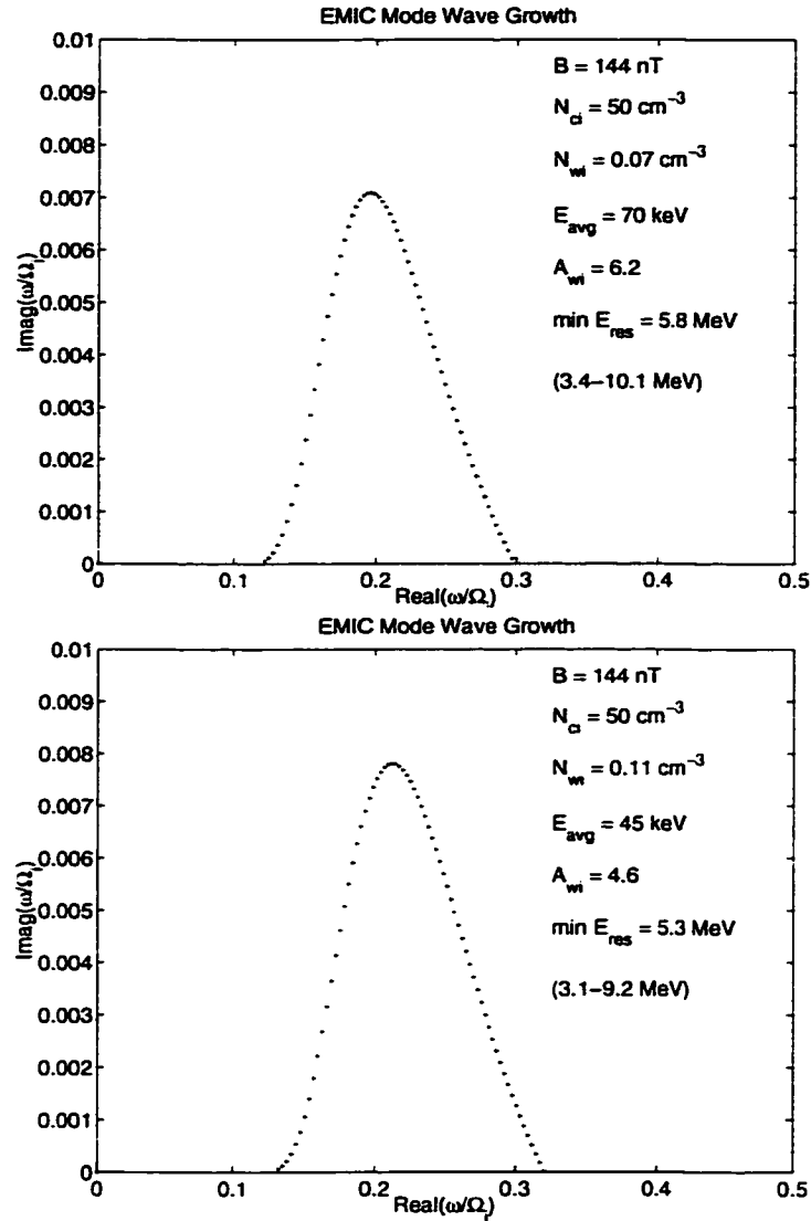
Figure 5.5: Electromagnetic ion cyclotron growth rate for parallel approximation. The top (bottom) panel shows growth rates corresponding to the conditions at the start (end) of the REP event predicted by the drift model.
