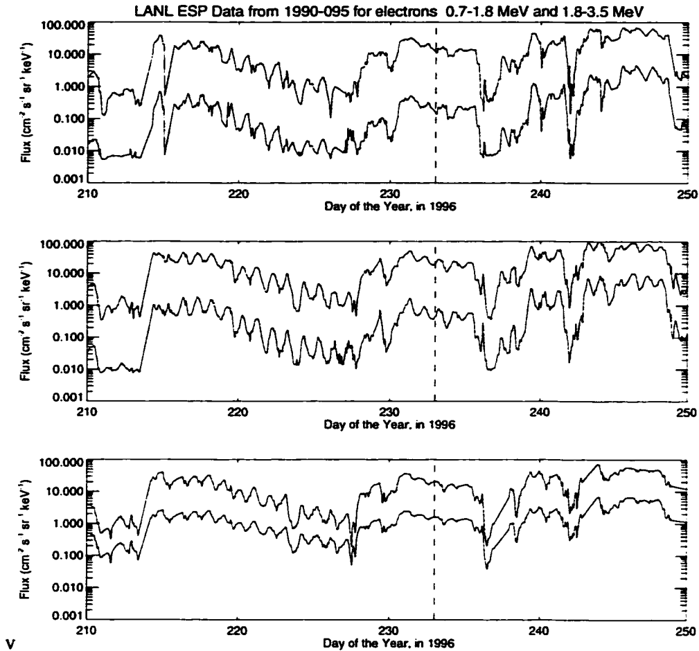
Figure 3.17: High energy electron data from the ESP instrument on the LANL geosynchronous satellites, courtesy of G. D. Reeves. The plot shows the entire month of August. Day 233 corresponds to August 20 and is indicated with a vertical dashed line.
