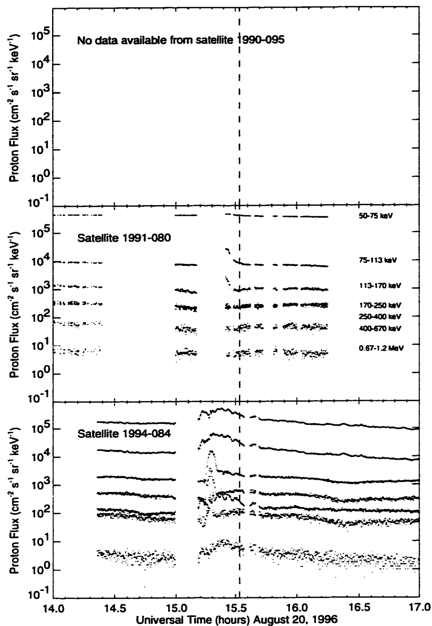
Figure 3.16: Proton data from the LANL geosynchronous satellites, courtesy of G. D. Reeves. All data are from the SOPA instrument. The substorm injection is most clearly visible in the lower energy (50-400 keV) channels of satellite 1994-084 starting at about 1512 UT. The satellite was close to the injection region, since very little energy dispersion can be seen these data. The 400-670 keV channel is contaminated with electrons. The start of the REP event at 1532 UT is indicated with a dashed vertical line.
