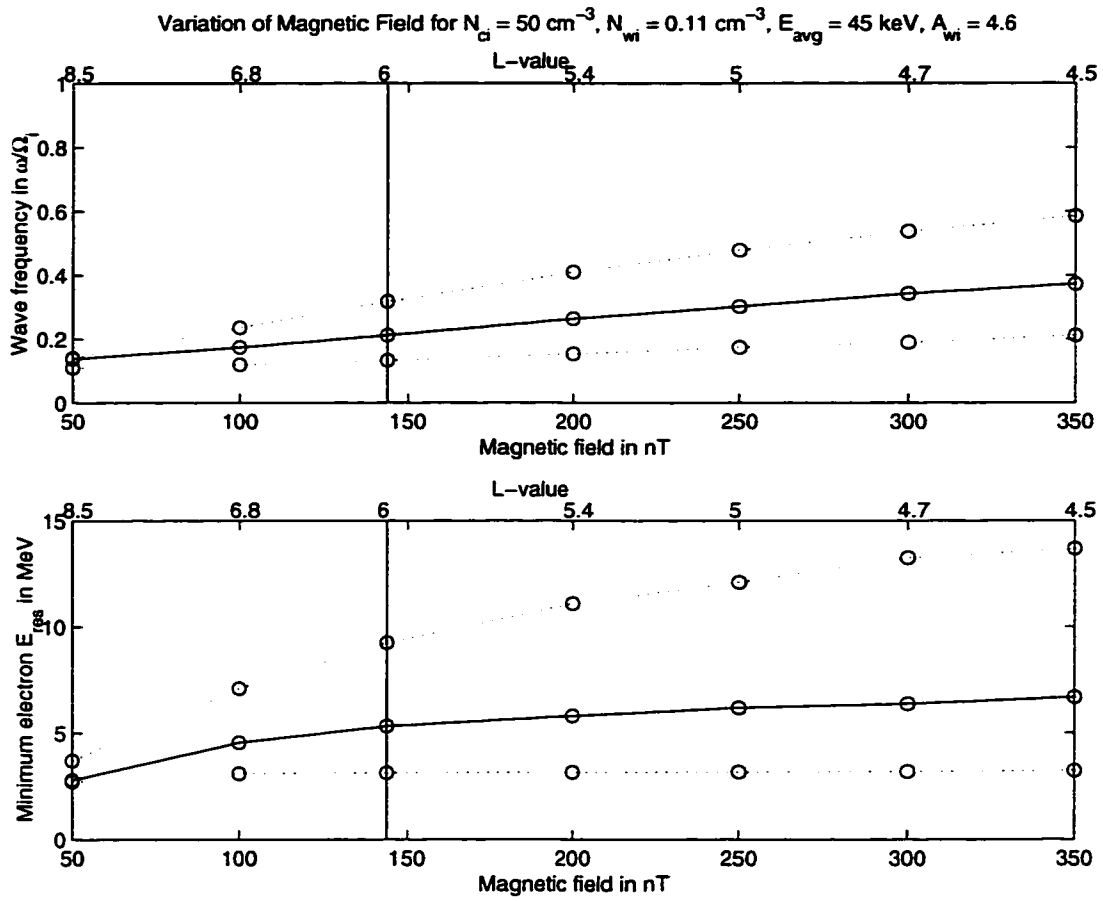
Figure 5.6: Wave frequency and electron resonance energy vs. magnetic field strength. The top axis of each panel shows the corresponding L-values and the vertical line shows the parameters used to determine the wave growth shown in the bottom of Figure 5.5.
