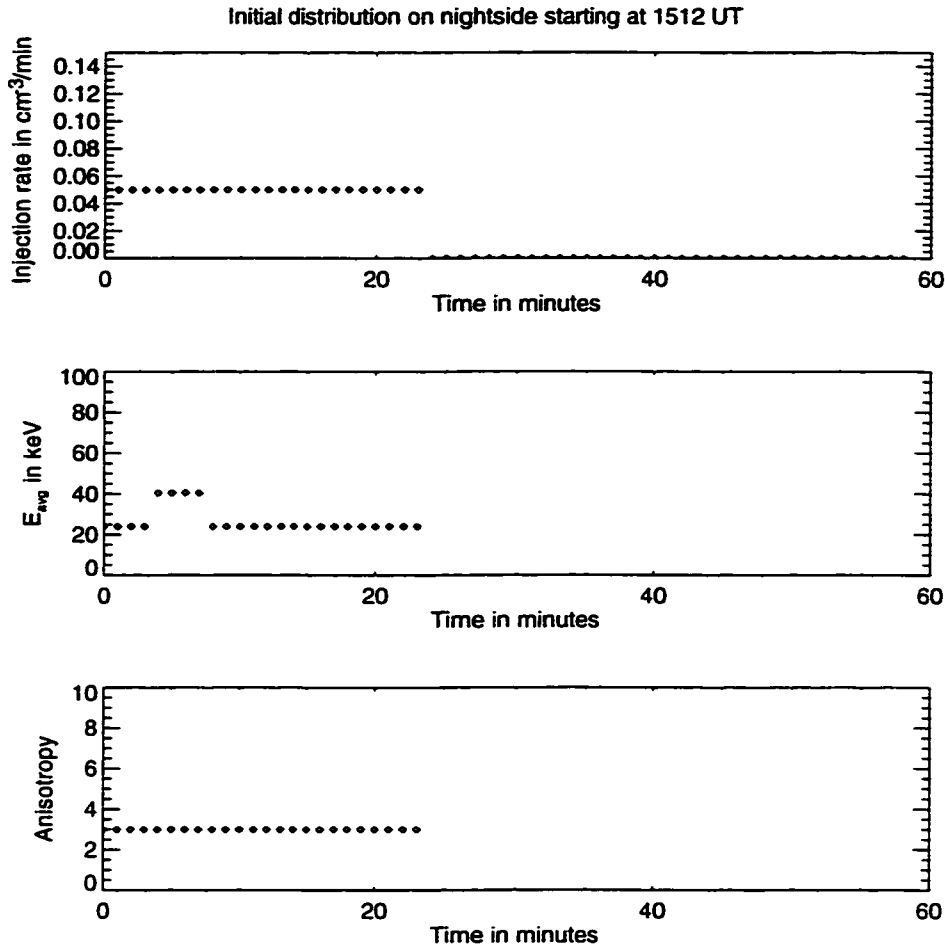
Figure 5.3: Initial nightside conditions for the injection rate, average energy and temperature anisotropy of the proton drift simulation.
