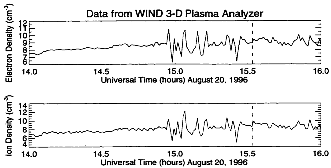
Figure 3.21: Particle data from the WIND spacecraft, from the CDA web site, courtesy of R. P. Lin, University of California at Berkeley. The start of the REP event at 1532 UT is indicated with a dashed vertical line.
