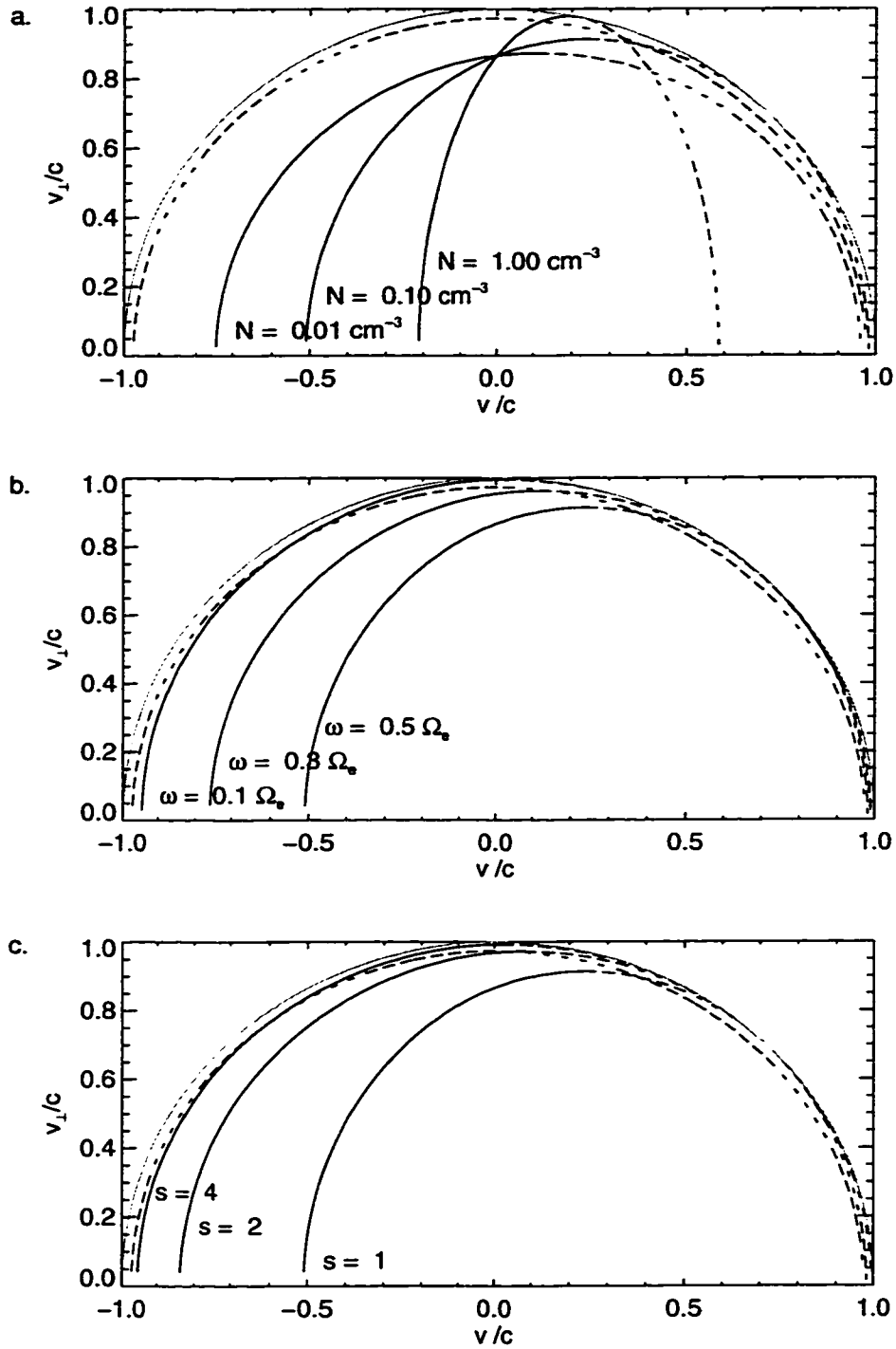
Figure 4.5: Variation in whistler resonance ellipse with a) density for |s| = 1 and \omega = 0.5\Omega_e , b) frequency for N = 0.1 \text{ cm}^{-3} and |s| = 1 , and c) harmonic for N = 0.1 \text{ cm}^{-3} and \omega = 0.5\Omega_e . The outer solid circle is where v = c and the inner dashed circle is for electrons of energy 1.7 MeV.
