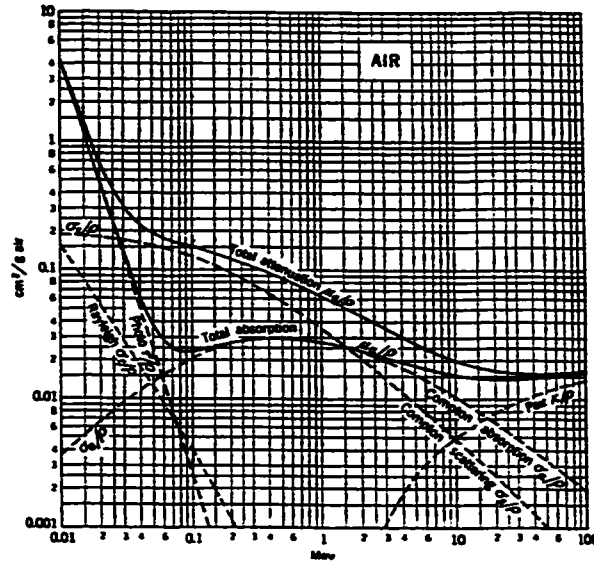
Figure 2.8: Mass attenuation coefficients for air, from Evans [1955].
