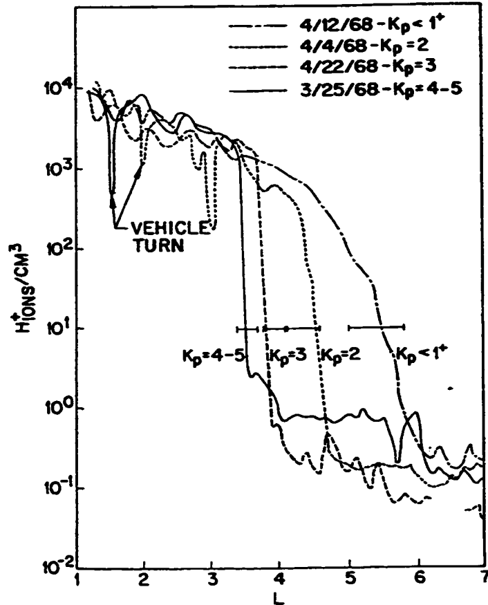
Figure 4.8: Typical nightside equatorial ion densities indicating plasmapause locations for various levels of magnetic activity [Chappell et al. , 1970].
