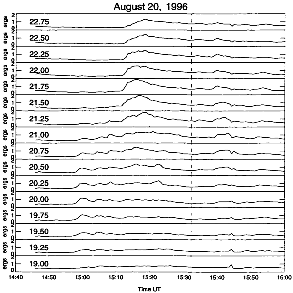
Figure 3.12: Energy input to the atmosphere measured in 15-minute pie slices in MLT by the UVI instrument. The vertical dashed line shows the start of the REP event at 1532 UT. The peak at 1544 UT corresponds to a camera platform shift and is not real.
