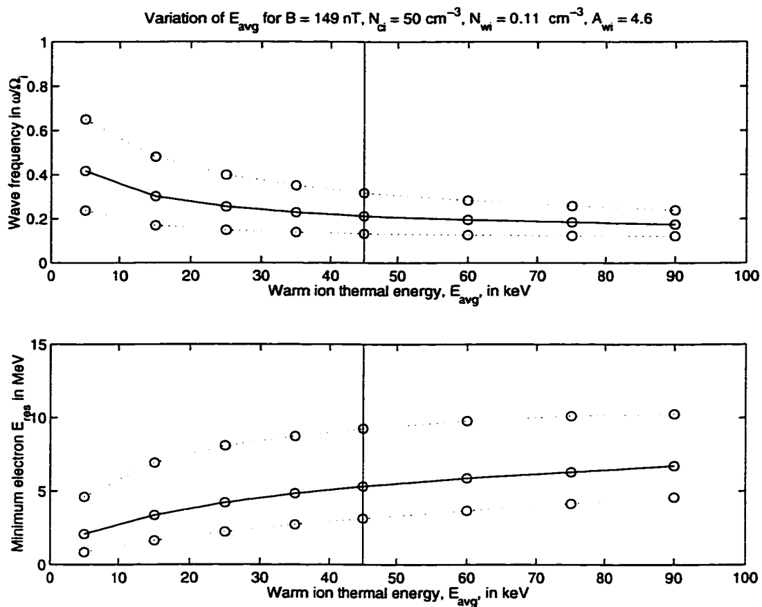
Figure 5.9: Wave frequency and electron resonance energy vs. warm ion average thermal energy. The vertical line shows the parameters used to determine the wave growth shown previously in the bottom of Figure 5.5.
