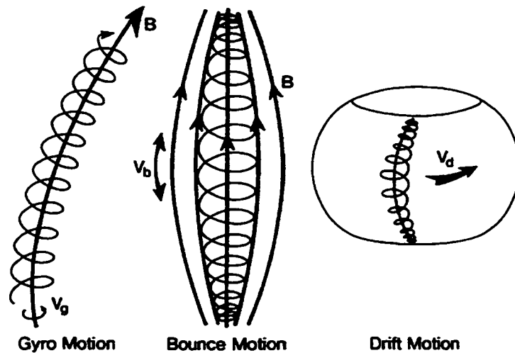
Figure 1.1: Three kinds of particle motion in a dipole magnetic field, from Kivelson and Russell [1995].
