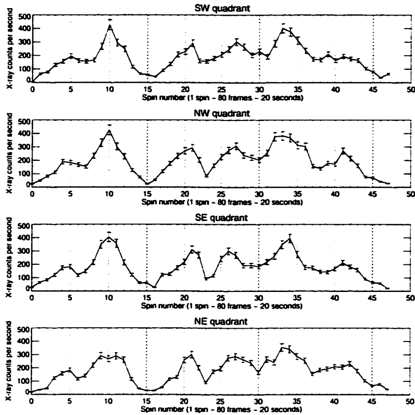
Figure 3.5: Background-subtracted X-ray count rate for each of the four quadrants of the X-ray imager during the REP event.
