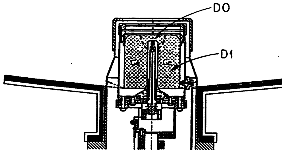
Figure 2.10: The germanium X-ray spectrometer, from Smith et al. [1995]. For the INTERBOA campaign, the lead collimator was much narrower, restricting the field of view to 90 degrees and only data from detector D1 was used.
