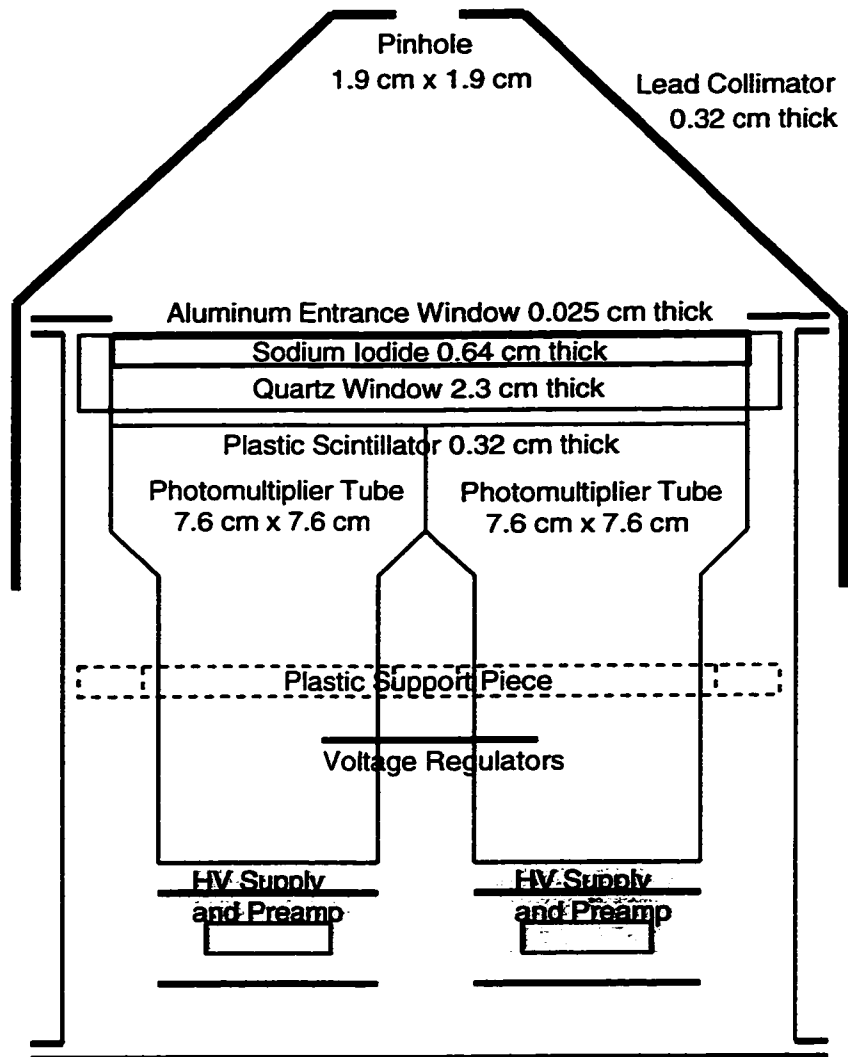
Figure 2.2: A cross-section of the X-ray imager camera unit.
