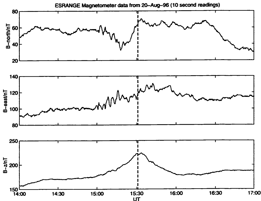
Figure 3.8: Magnetometer data from Esrangle, courtesy of L. E. Sarri. The northward component shows a small magnetic bay, and the eastward component shows fluctuations that are strongest about half an hour before the REP event. The start of the REP event at 1532 UT is indicated with vertical dashed lines.
