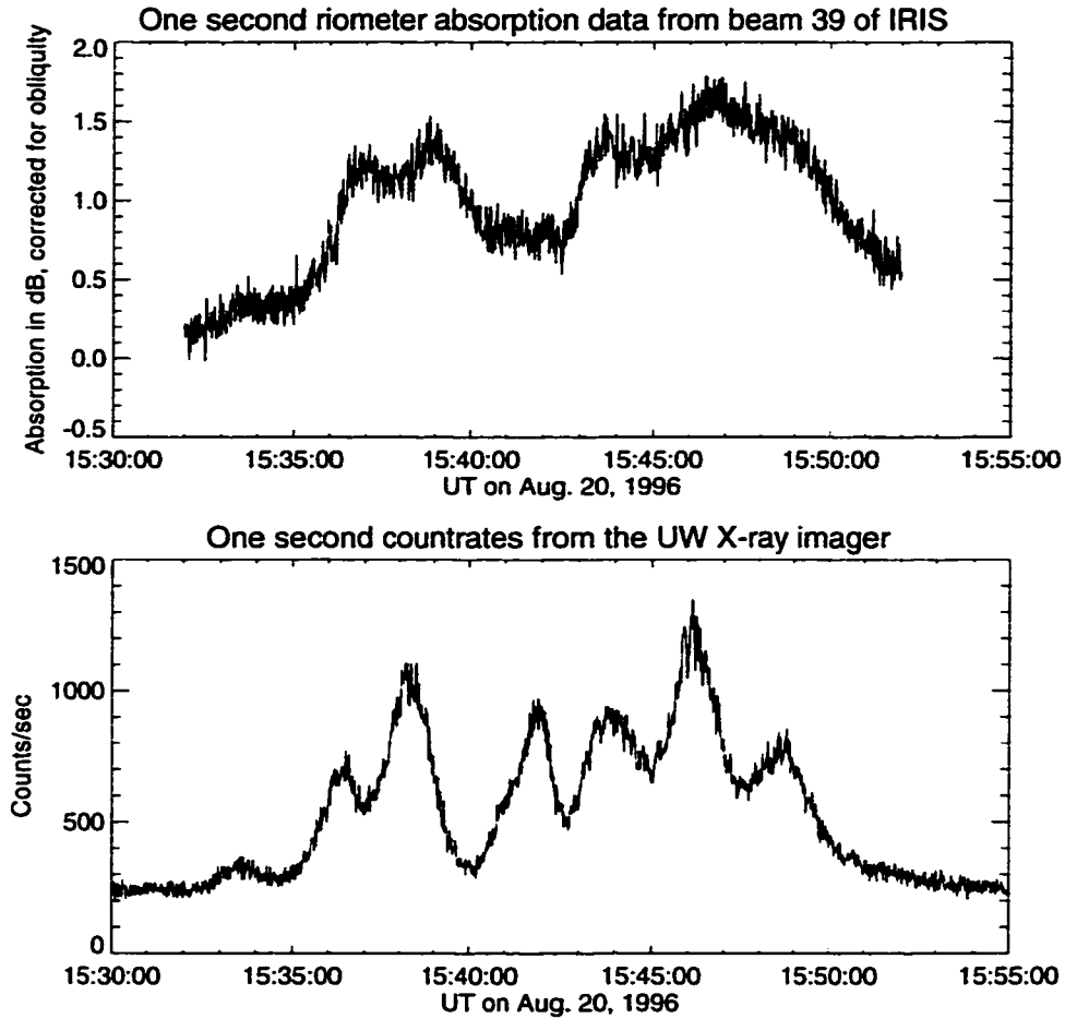
Figure 3.10: One-second riometer absorption data from the Imaging Riometer for Ionospheric Studies (IRIS) at Kilpisjärvi, Finland. These data are from beam 39, which is in the lower (southern) middle of the 49-beam array. At the 60 km projection altitude, this beam is close to the center of the X-ray imager field of view.
