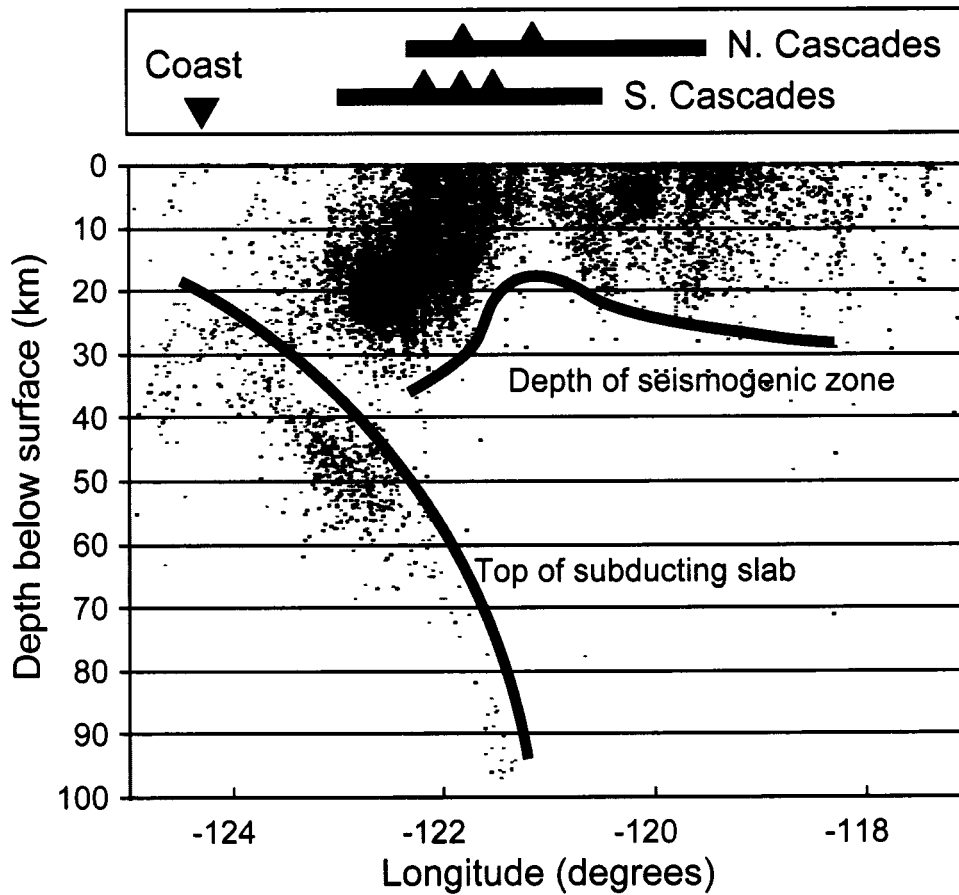
Figure 4.5: Earthquake focal depths (in km) between 45^{\circ} N and 49^{\circ} N latitude as a function of longitude (decimal degrees) in Washington State, 1965-2006 (data from Pacific Northwest Seismograph Network). Earthquakes with M > 2 ( N = 8,910 ) are shown as black dots, earthquakes with 1 < M < 2 ( N = 17,387 ) are shown as gray dots. Top panel shows approximate longitude of the coast (downward triangle), the western and eastern limits of the Cascades (horizontal bars), and the Quaternary volcanoes (triangles).
