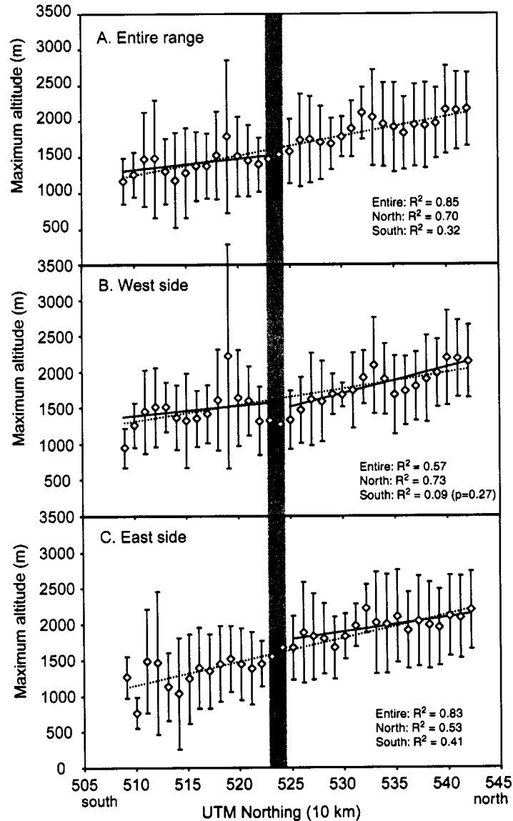
Figure 2.4: Maximum altitudes (diamonds) averaged across 10-km-wide latitudinal bins for: A, the entire range; B, west of the range crest; and C, east of the range crest. Error bars indicate the 1\sigma standard deviation. The vertical gray bar denotes the approximate latitude of Snoqualmie Pass, dividing the range into northern (right) and southern (left) regions. Least squares linear regressions for the average maximum altitude for the entire (dashed line), northern (solid line), and southern (solid line) areas of the range are also shown (note: if the regression for a subregion overlaps the regression for the entire range, only the latter is shown). All p-values are < 0.01 unless noted.
