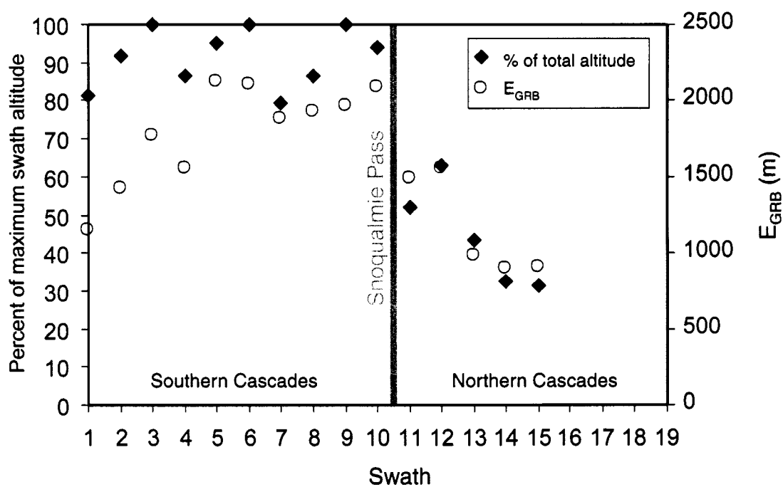
Figure 2.10: Open circles show the elevation of the highest exposure of GRB ( E_{GRB} ) in each swath, black diamonds show E_{GRB} as a percentage of the maximum elevation within each swath, excluding Quaternary volcanoes. Note there are no GRB exposures in swaths 16 to 19.
