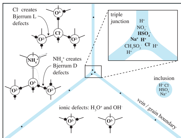
Figure 1.1: Illustration of the conduction mechanisms that are present in both pure and impurity-laden polar ice. The small circles adjacent to O^{2-} or O^{2-} -replacing ions represent H^+ ions. Blue represents water, and white represents the ice lattice.
