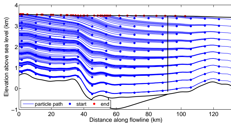
Figure 5.4: Modeled reversed particle paths from every fifth point in the two-dimensional, depth-normalized grid along the Vostok flowline.
