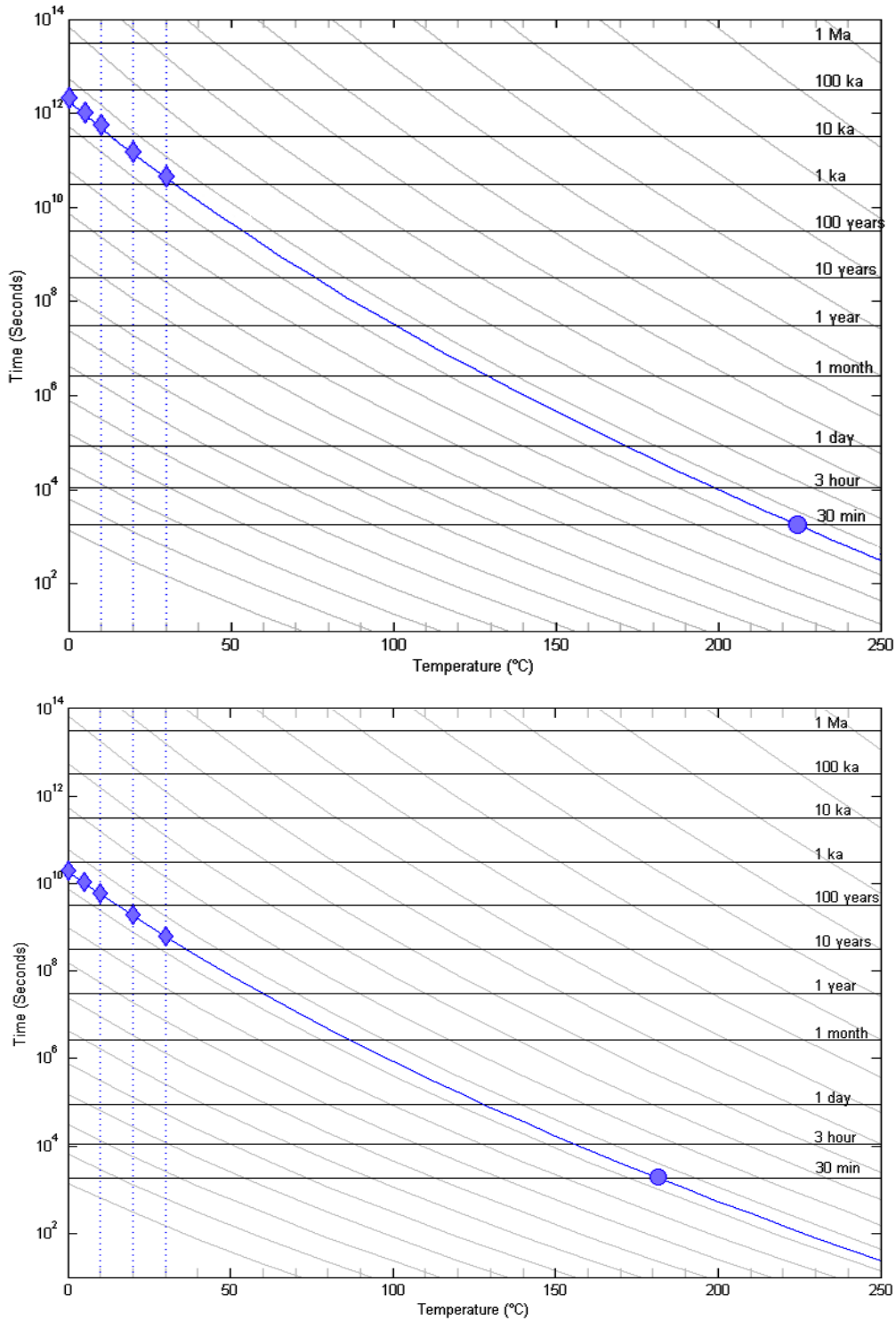
Figure 14: Following Middleton and Schmidt (1982) time-temperature nomographs, TVRM laboratory acquisition conditions shown as a circle with a suite of possible field acquisition temperatures represented as diamonds, for A) Mountain Home and B) Rat Creek. Assigning a field acquisition temperature between 0°C and 5°C results in a moraine age most in agreement with cosmogenic results of Porter and Swanson (2003).
