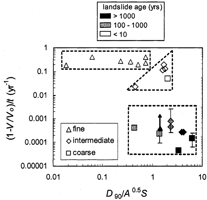
Figure 4.8: Plot of the normalized, long-term sediment export rate [(1-V/V_0)/t] versus the bed surface-based capacitance index (D_{90}/A^{0.5}S) . Symbology is the same as in Figure 4.7. The arrow on the black triangle designates a minimum age for the lower Church Mt. landslide, where V=0 . Dashed boxes define three landslide groups based on age and grain-size classification.
