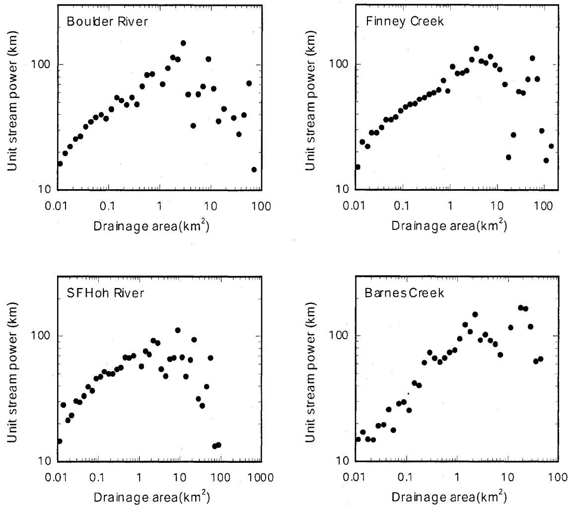
Figure 2.9: Log-bin-averaged index of unit stream power [(1/c)A^{(1-b)}S] derived from DEMs versus drainage area.
